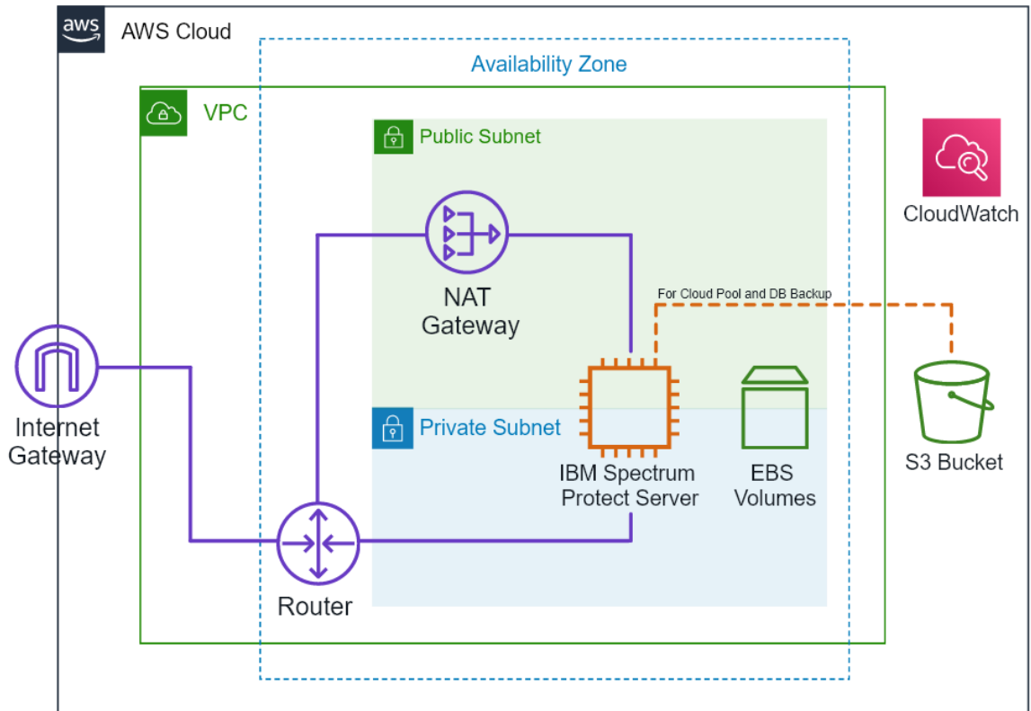
Figure 8: Architecture after deployment of IBM Spectrum Protect to a new VPC
