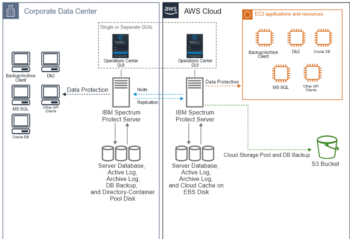
Figure 10: Architecture for node replication with one AWS and one on-premises instance
