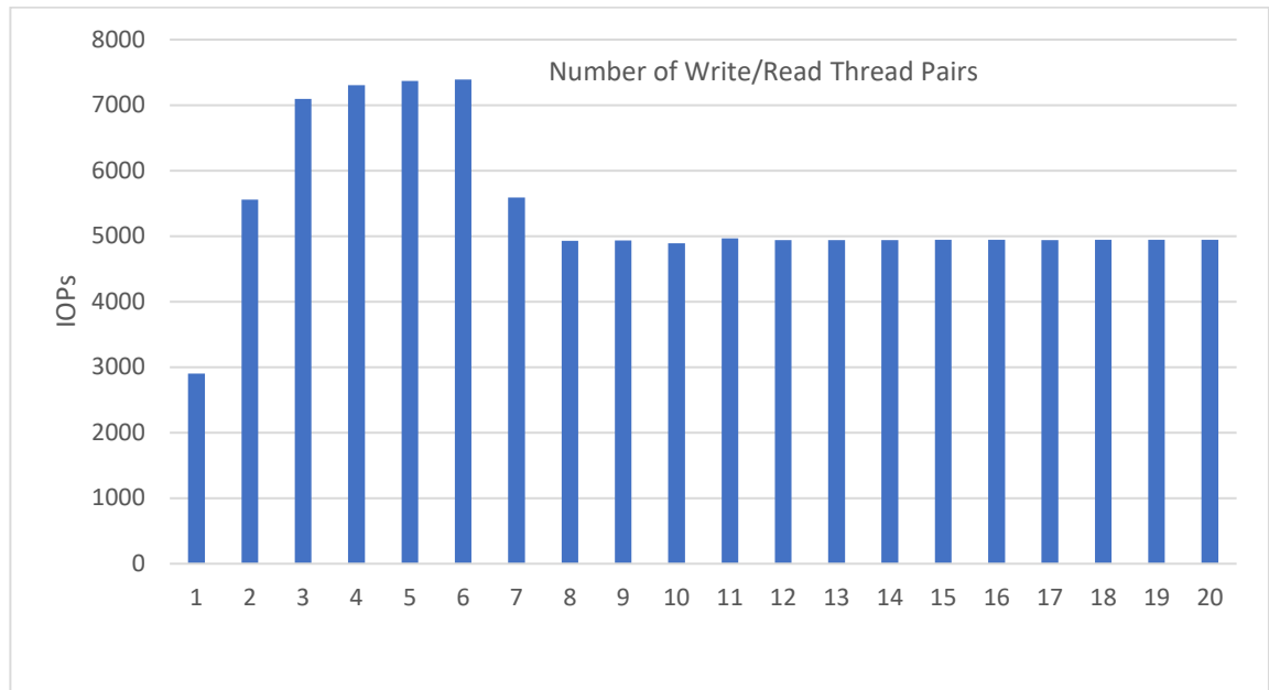
Figure 18: AWS small configuration; database volume average IOPS; 8 KiByte random writes/reads
