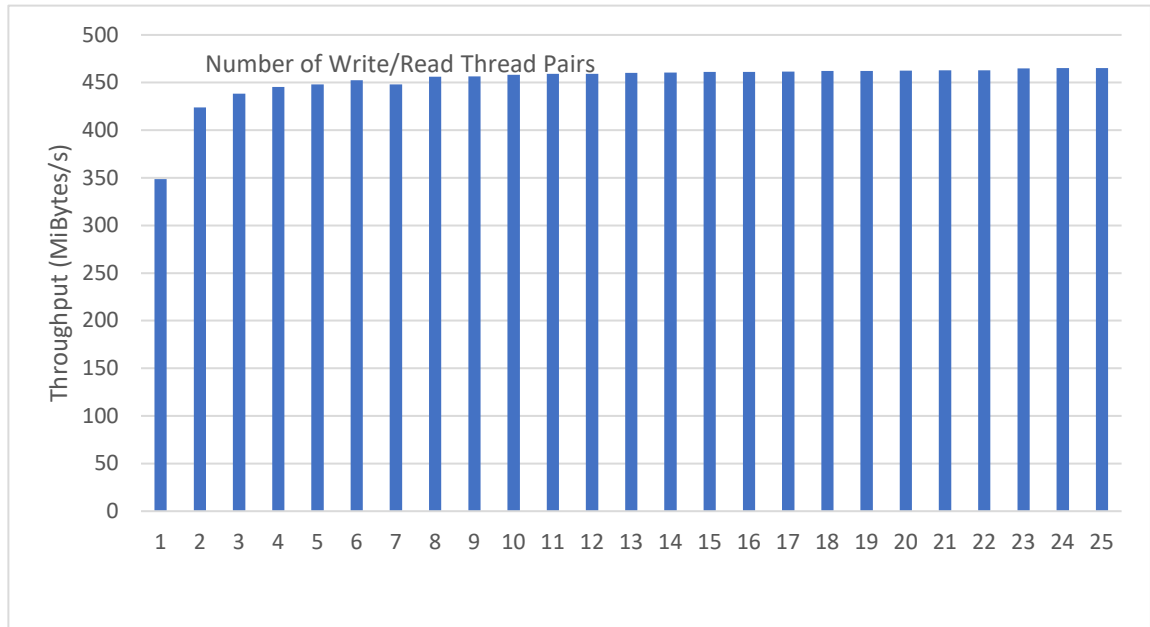
Figure 16: AWS medium configuration; cloud cache volume average throughput; mixed 256 KiByte writes and reads
