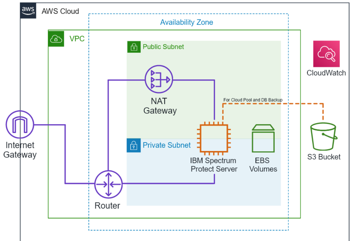
Figure 7: Architecture after deployment of IBM Spectrum Protect to an existing VPC
