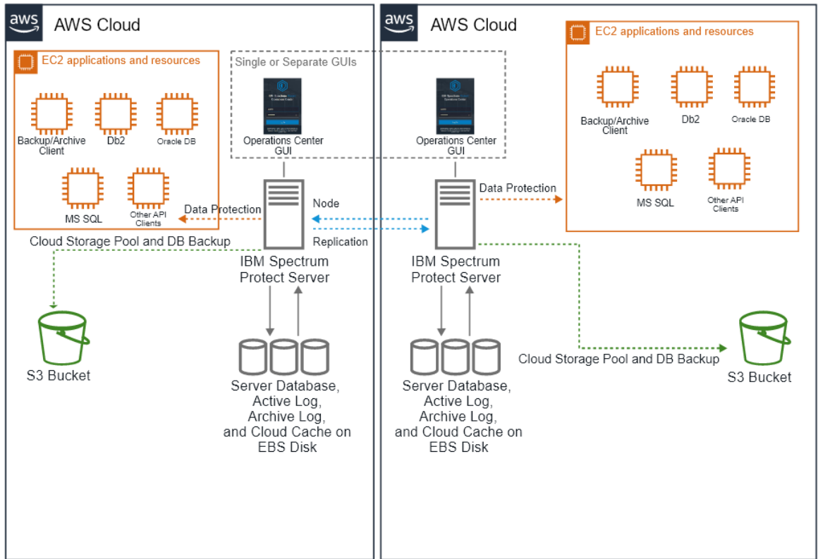
Figure 9: Architecture for node replication between two servers in separate AWS-hosted instances
