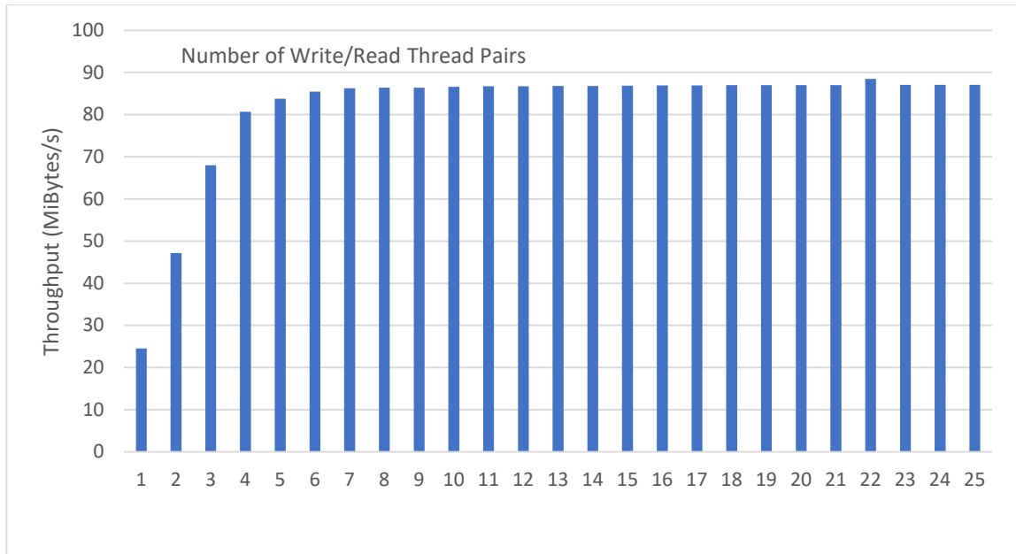
Figure 14: AWS medium configuration; database volume average throughput; 8 KiByte random writes/reads
