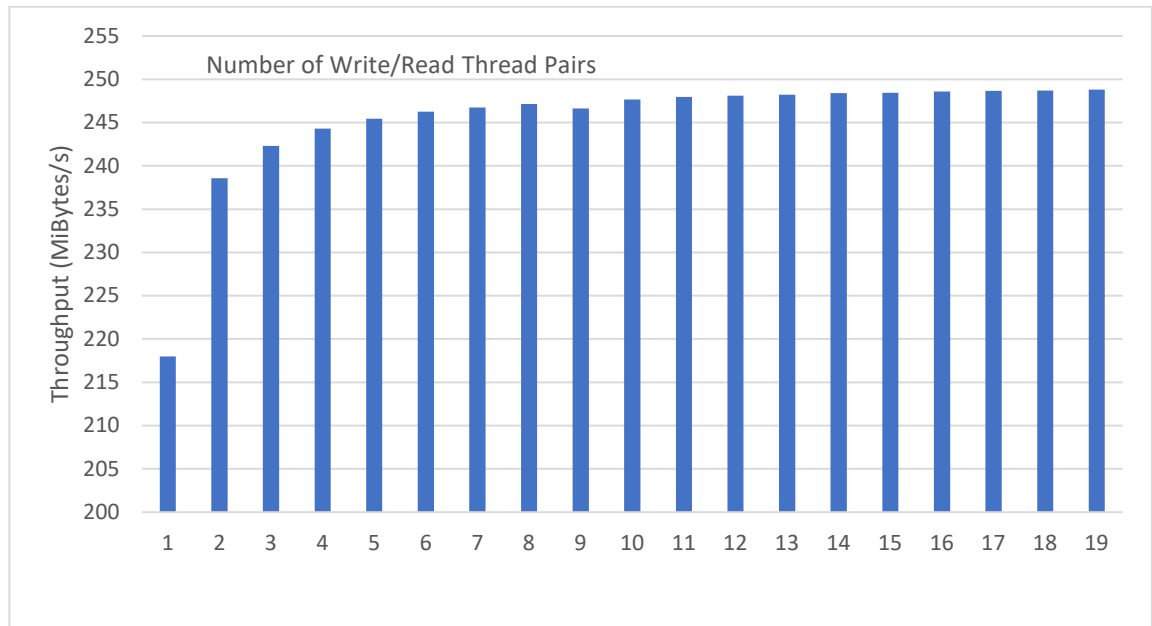
Figure 19: AWS small configuration; cloud cache volume average throughput; mixed 256 KiByte writes/reads
