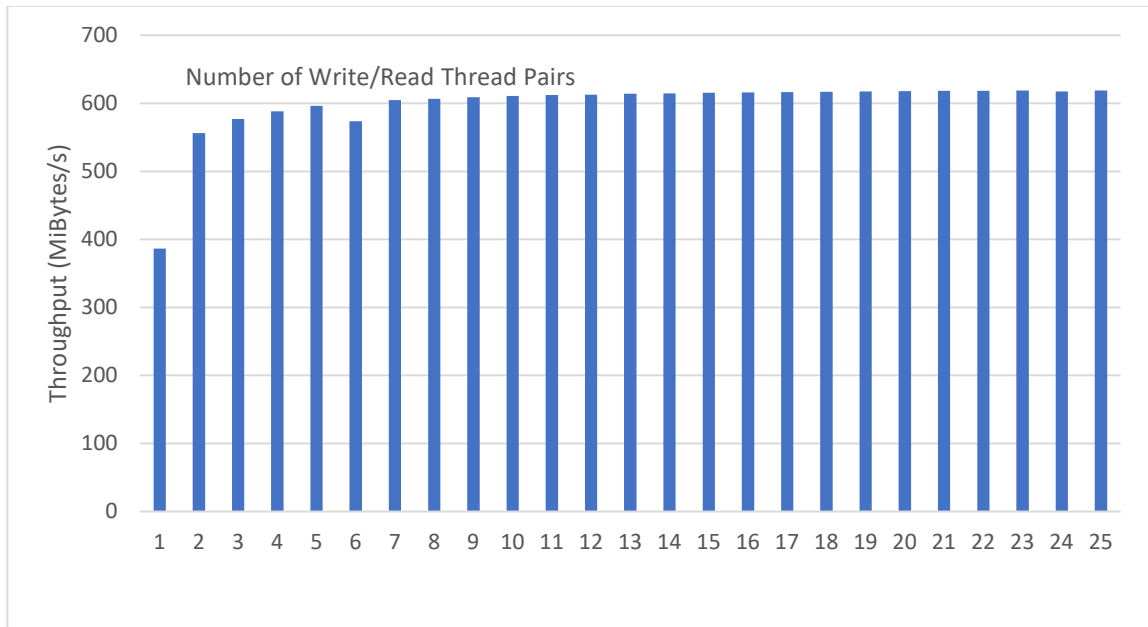
Figure 13: AWS large configuration; cloud cache volume average throughput; mixed 256 KiByte writes and reads
