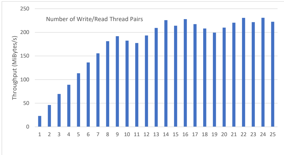
Figure 11: AWS large configuration; database volume average throughput; 8 KiByte random writes/reads
